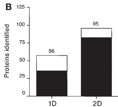
Figure 2. Identifying proteins in the yeast ribosome complex using DALPC. (A) Cumulative number of unique peptides identified from a digested ribosomal 80S complex using 1D liquid chromatography (LC) and 2D LC coupled to a mass spectrometer. The numbers enclosed in the 2D bracket are the salt displacement step gradients used in the experiment (see Experimental protocol). The cumulative total of peptides identified after each DALPC cycle is shown. The numbers above the columns are the total numbers of unique peptides identified. Identical amounts of digested proteins were used for both experiments. (B) Number of proteins identified starting with identical amounts of trypsin-digested ribosomal proteins in the 1D and 2D chromatography experiments. The number of proteins identified based on two or more unique peptide sequences is shown in black. The numbers above the
