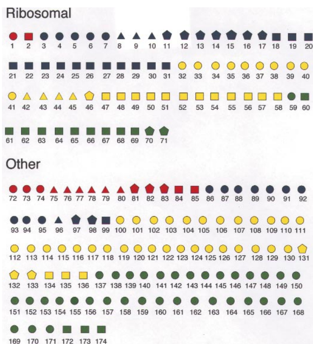
Figure 3. Identifying ribosomal proteins in a total yeast extract using DALPC. A 375 µg aliquot of an acidified total yeast protein digest was analyzed using the DALPC conditions described in Experimental protocol, except 21 salt step gradients were used. The meanings of the icons are explained in Figure 2C and the protein names have been put into a web site 32 . The identified proteins have been grouped into two classes, ribosomal and other. The SCX step gradients were: 0%, 0–10%, 10–12.5%, 12.5–15%, 15–17.5%, 17.5–20%, 20–22.5%, 22.5–25%, 25–27.5%, 27.5–30%, 30–32.5%, 32.5–35%, 35–37.5%, 37.5–40%, 40–50%, 50–60%, 60–70%, 70–80%, 80–90%, 90–100% of SCX-B, and 100% SCX-C.
