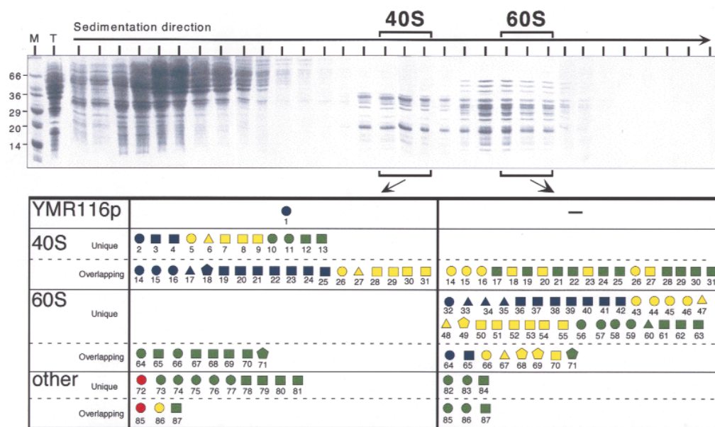
Figure 5. Localizing YMR116p to the yeast 40S ribosomal subunit. A Coomassie brilliant blue-stained 15% SDS-PAGE gel of sucrose-gradient fractions of a total yeast lysate. 40S and 60S are pooled ribosomal subunit fractions. (M, protein standards; T, protein lysate layered on the top of the sucrose gradient). Aliquots of 0.2 and 0.25 \mu g from the digested and desalted 40S and 60S subunit fractions, respectively, were analyzed using the integrated DALPC conditions described in Experimental protocol. The table shows the proteins identified in the fractions. The identified proteins have been divided into four classes (YMR116p, 40S, 60S, and other), and each class has been subdivided into proteins unique to a fraction or proteins identified in both fractions. The meaning of the icons is explained in Figure 2C, and the protein names have been put into a web site 32 .
