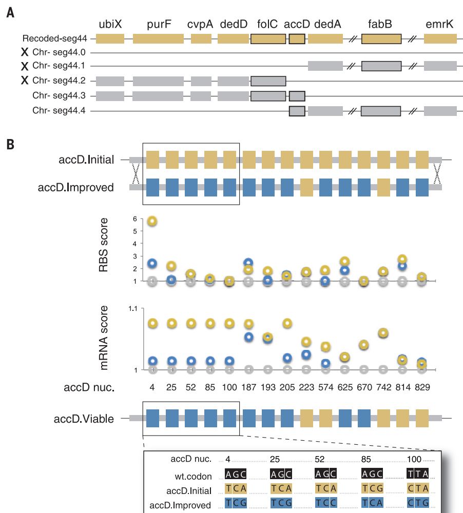
Fig. 4. Troubleshooting lethal design exceptions. (A) Recoded segment 44 (orange) did not support cell viability upon deletion of the corresponding chromosomal sequence (Chr-seg44.0). The causative recoded gene accD was identified by successive chromosomal deletions (Chr-seg44.1-4; "X," nonviable). Essential genes are framed. (B) \lambda -Red recombination was used to exchange lethal accD sequence ( accD.Initial , recoded codons in orange) with an alternative recoded accD sequence ( accD.Improved , alternative codons in blue). mRNA structure and RBS motif strength were calculated for both sequences. Wild type shown in gray. accD nuc is the first position in each recoded codon. The resulting viable sequence ( accD.Viable ) carried codons from both designs. Full sequences are provided in fig. S11. mRNA and RBS scores are the ratio between predicted mRNA folding energy (kcal/mol) (37) or predicted RBS strength (38) of recoded and nonrecoded codon.
